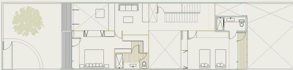
PLANTA ALTA / SECOND FLOOR
